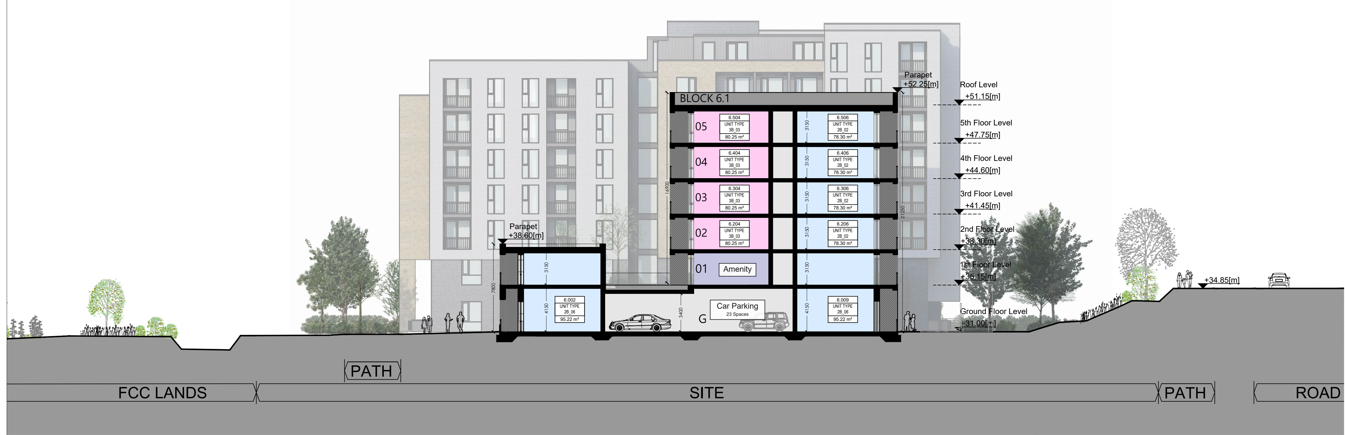
Section AA - Block 6 Scale 1:200 @A1
