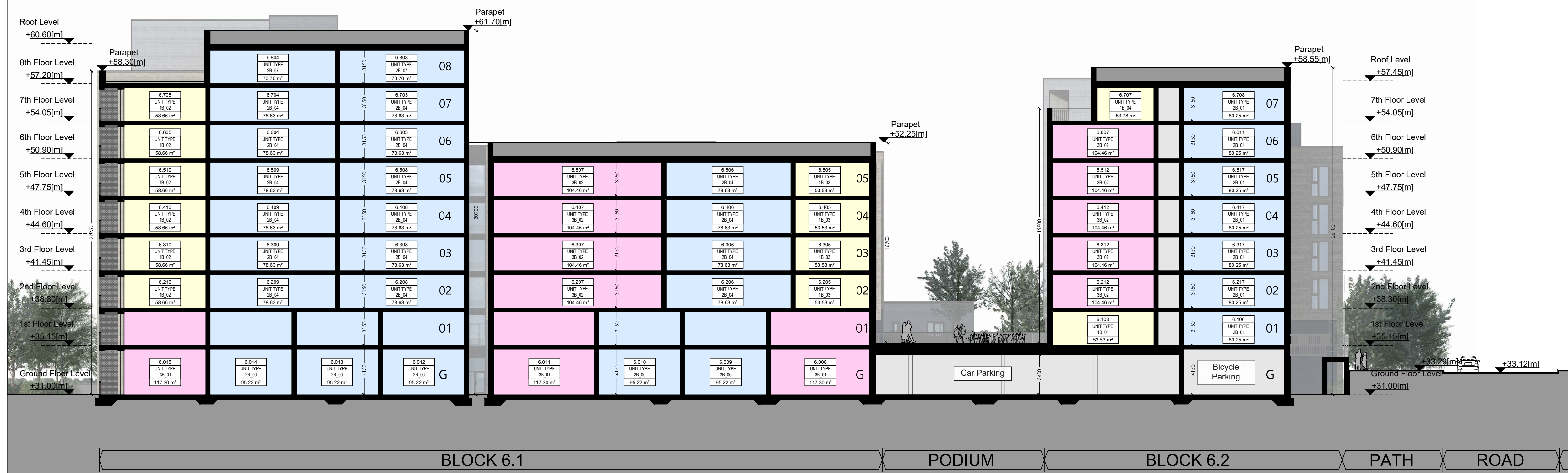
Section BB - Block 6 Scale 1:200 @A1
